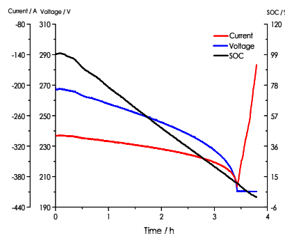
2、额定容量曲线 Rated Capacity Curve
